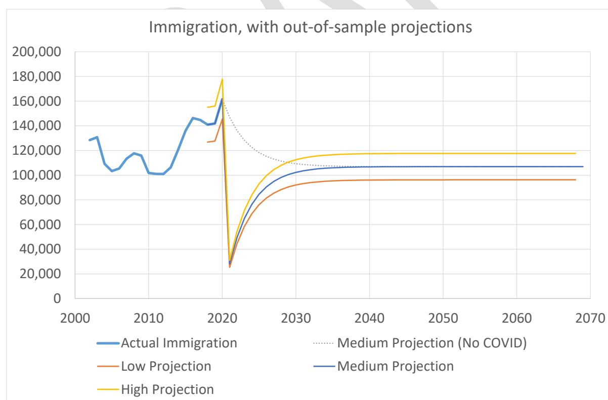
Figure 2: Actual and projection national-level immigration flows, 2002-2068
