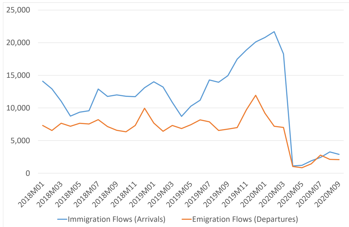
Figure 5: Monthly international migration flows, 2018-2020
